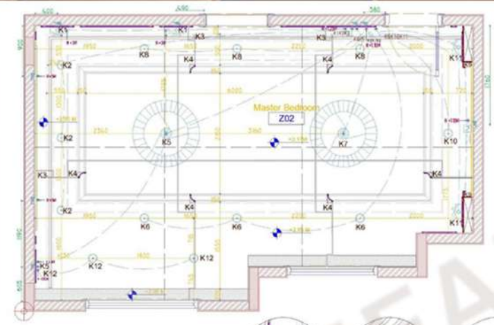
Z02 ELEC - PLANS PLN MASTER BEDROOM
